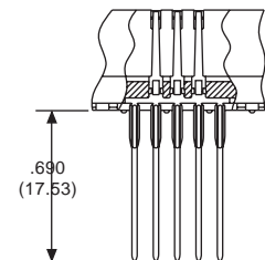
Code 4
