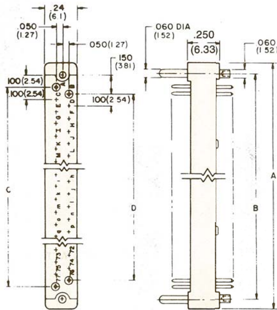
PLUG MEETS MIL-C-55302/5
